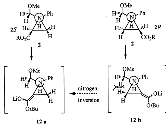
Figure 2. Relative stabilities of the enolates 12a and 12b
