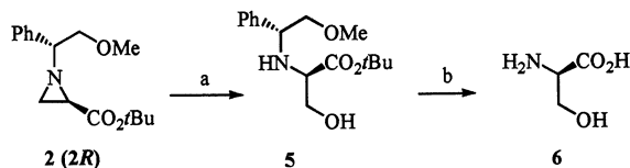
Scheme 3. Reagents and conditions: a) 20% aq. HClO 4 , 80 °C, 15 h, 48%; b) H 2 , Pd(OH) 2 , EtOH/H 2 O (1:1), 100%
