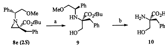
Scheme 5. Reagents and conditions: a) 20% aq. HClO 4 , 80 °C, 3 h, 31%; b) H 2 , Pd(OH) 2 , EtOH/H 2 O (1:1), 100%
